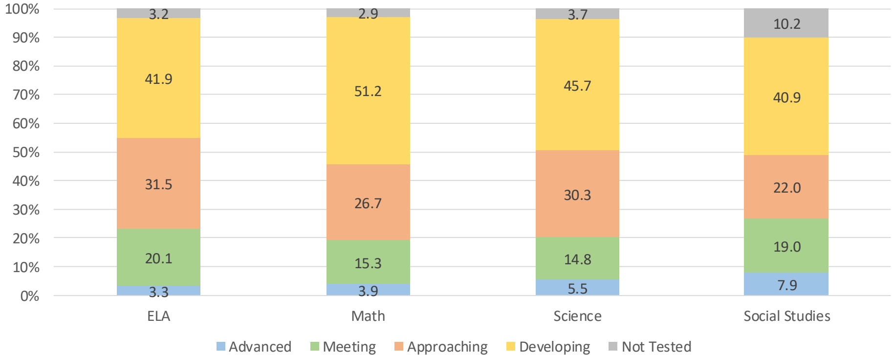
2023-2024 Wisconsin Forward Exam Performance by Category
