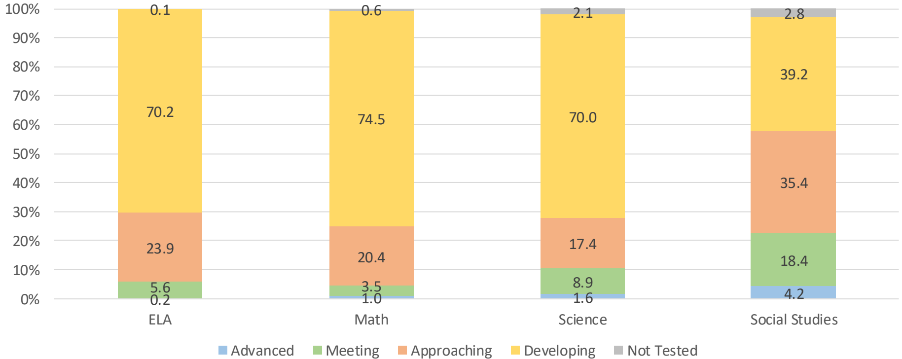
2023-2024 DLM Performance by Category
