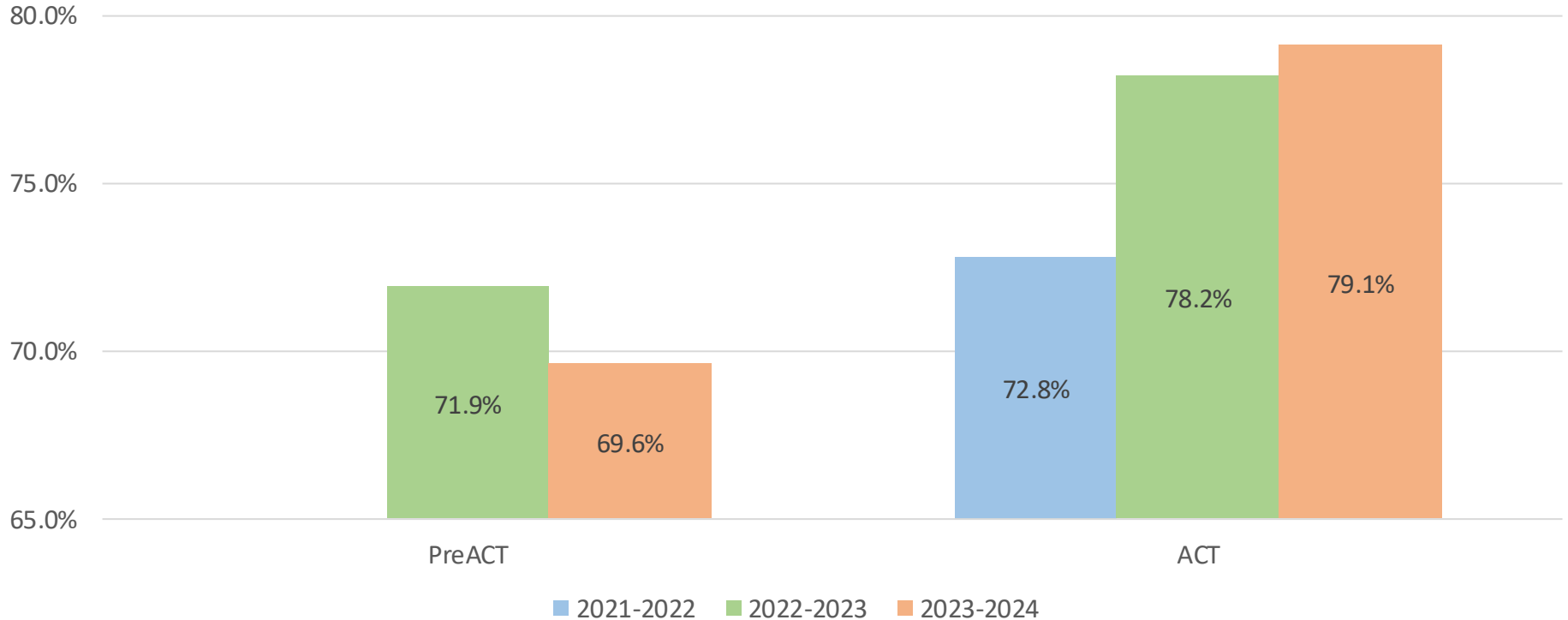
2023-2024 PreACT and ACT Test Completion
