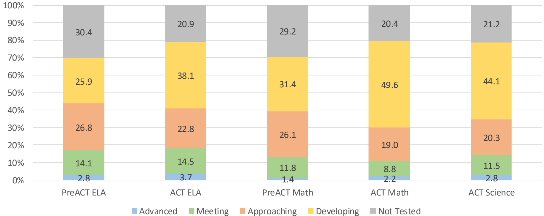
2023-2024 PreACT and ACT Performance by Category
