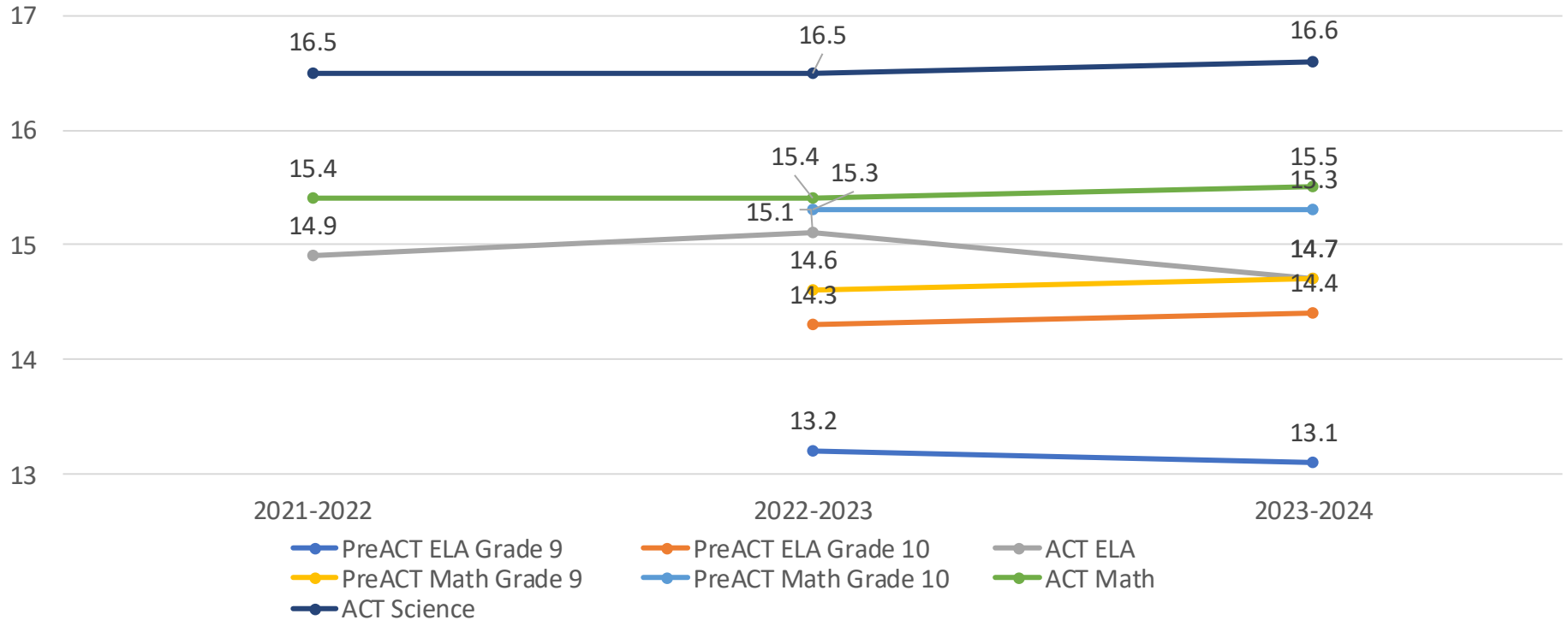
2023-2024 PreACT and ACT Average Score Trend
