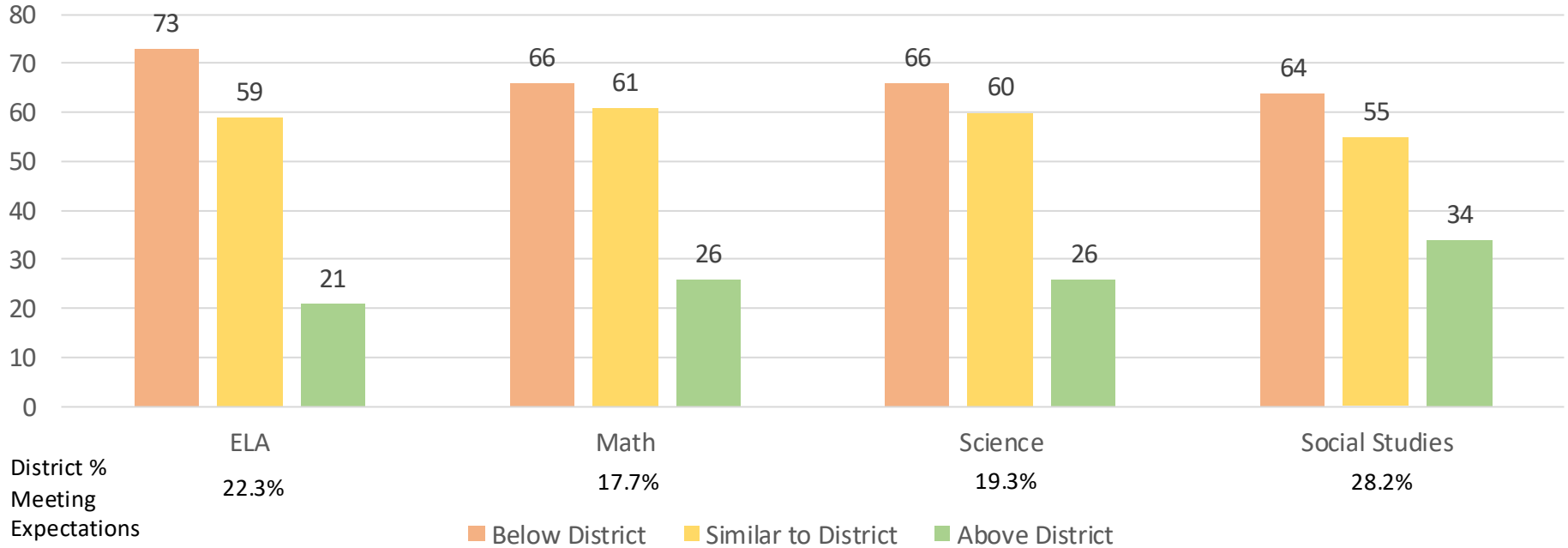
WSAS Distribution of Schools
